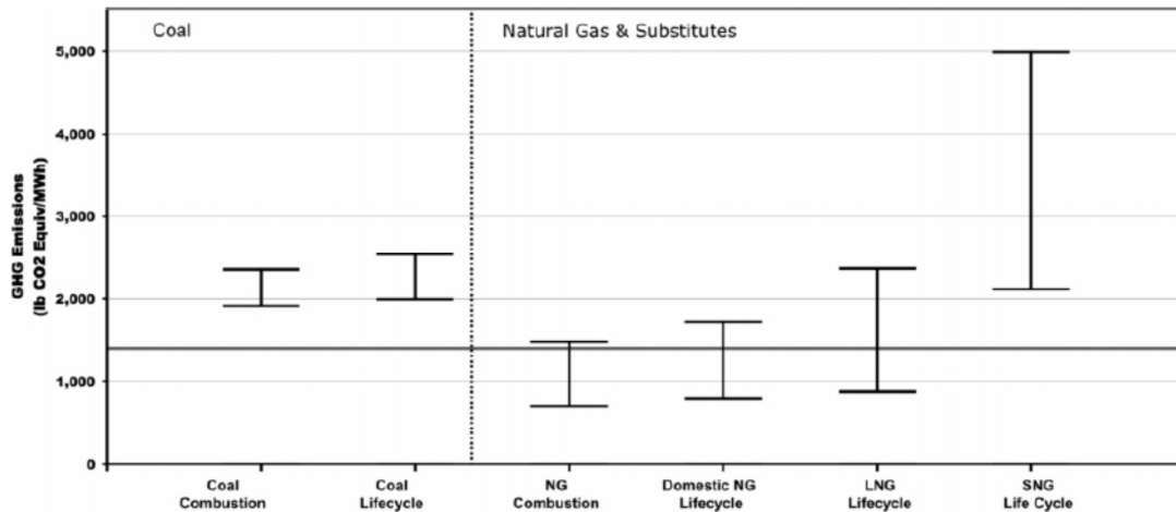
Figure 3: Life-Cycle Emissions of LNG, Natural Gas, and Coal in Electricity Generation 239
