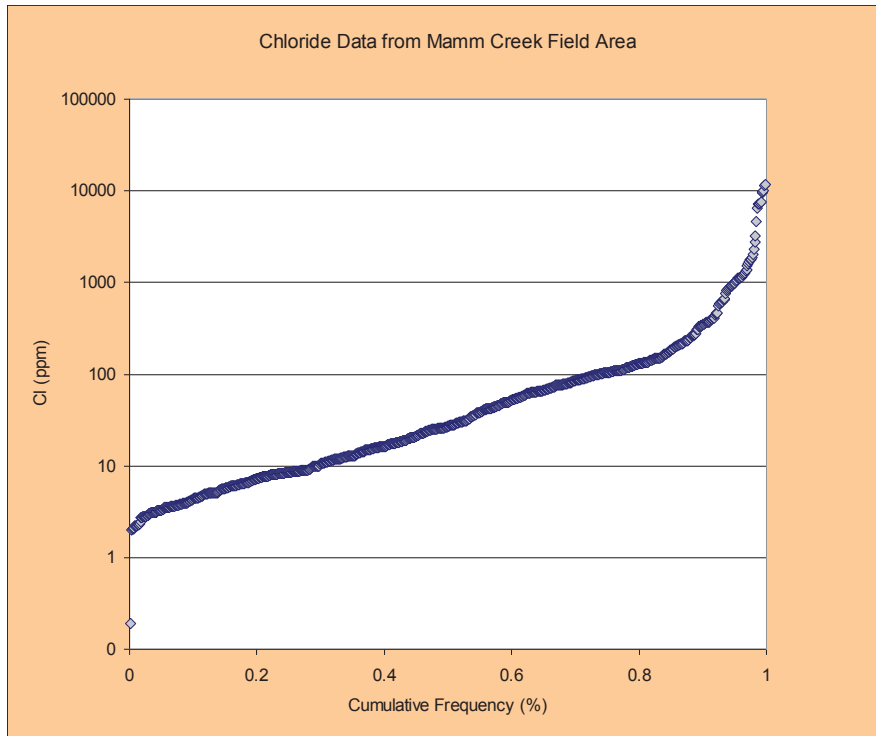
Figure 12. Cumulative frequency diagram for chloride content in water samples from the Mamm Creek Field area.
